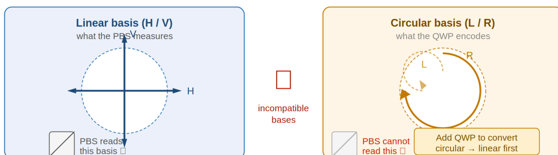
Fig 4.2 — Basis incompatibility. The PBS measures H/V only. Circular polarization requires a QWP to convert before the PBS can read it.
