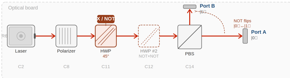
Fig 6.1 — Lab 6 beam path. HWP at 45^\circ = NOT gate X (red). HWP #2 (dashed) tests NOT \times NOT = I.
