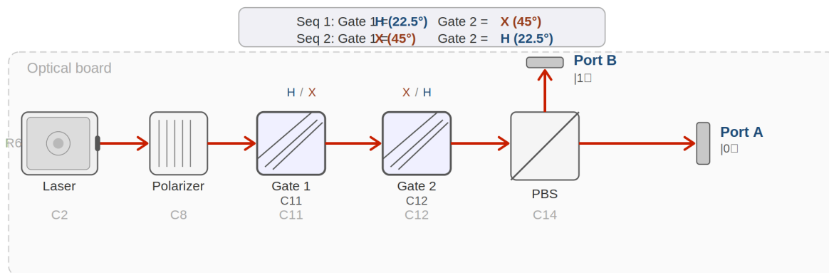
Fig 8.1 — Lab 8 beam path. Two HWPs in series. Gate assignments swap between Sequence 1 and Sequence 2.
