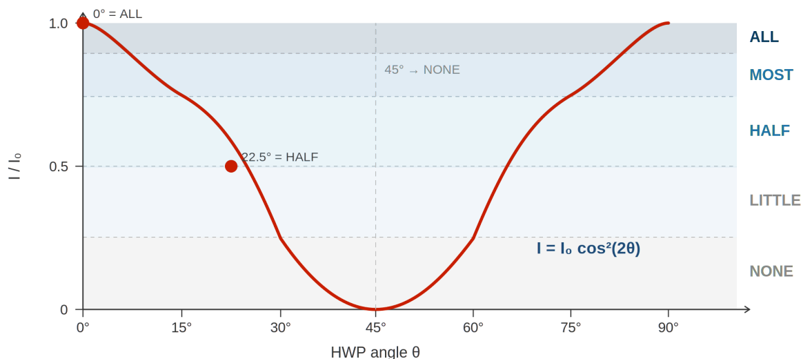
Fig 2.2 — Malus's Law with visual scale overlay. Predict your table entries from this curve before rotating.
