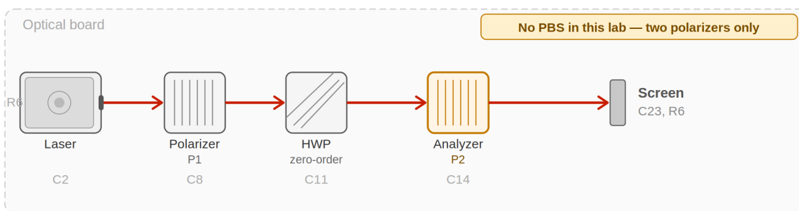
Fig 7.1 — Lab 7 beam path. Two polarizers — no PBS. The analyzer (amber) measures HWP phase output.
